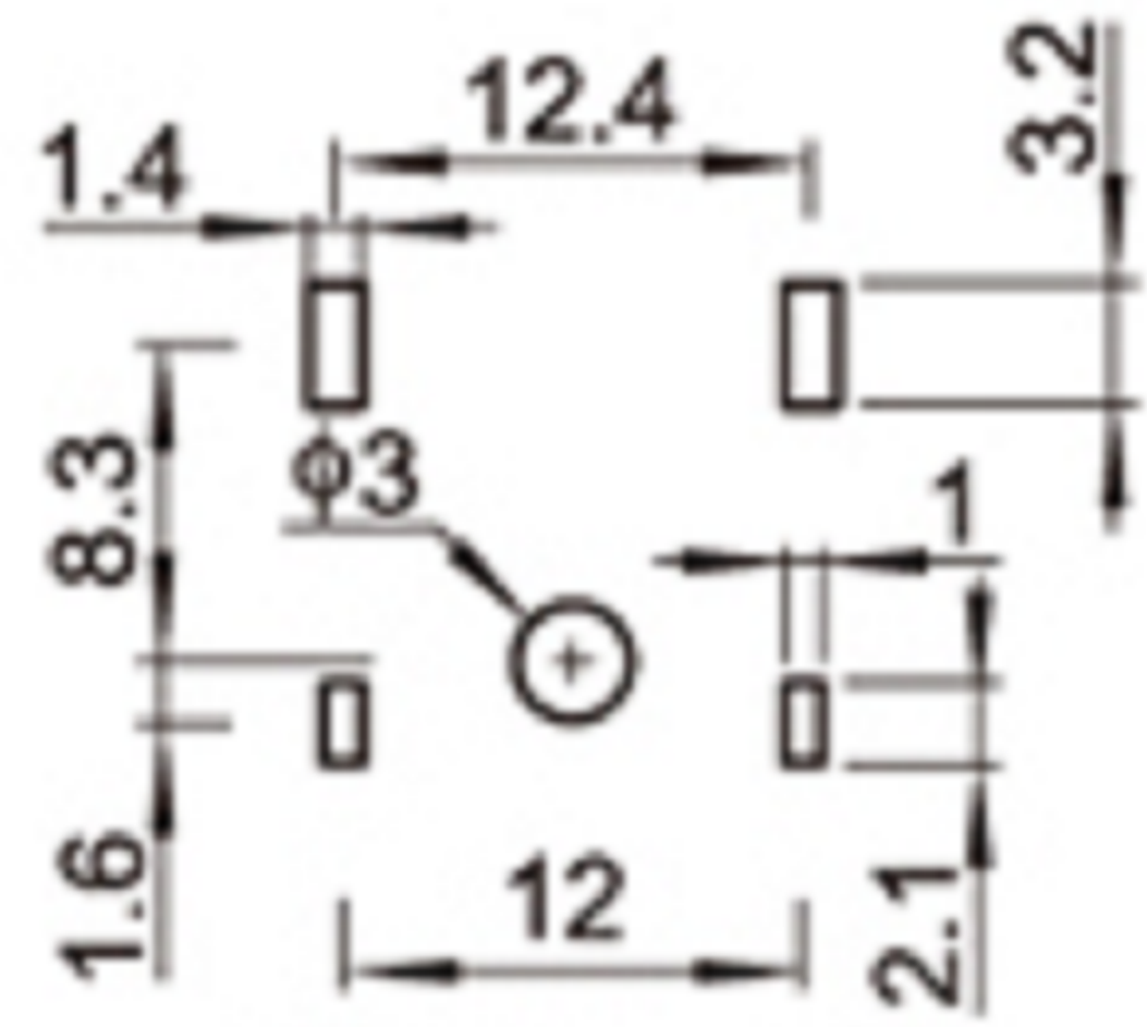
PANEL Layout
