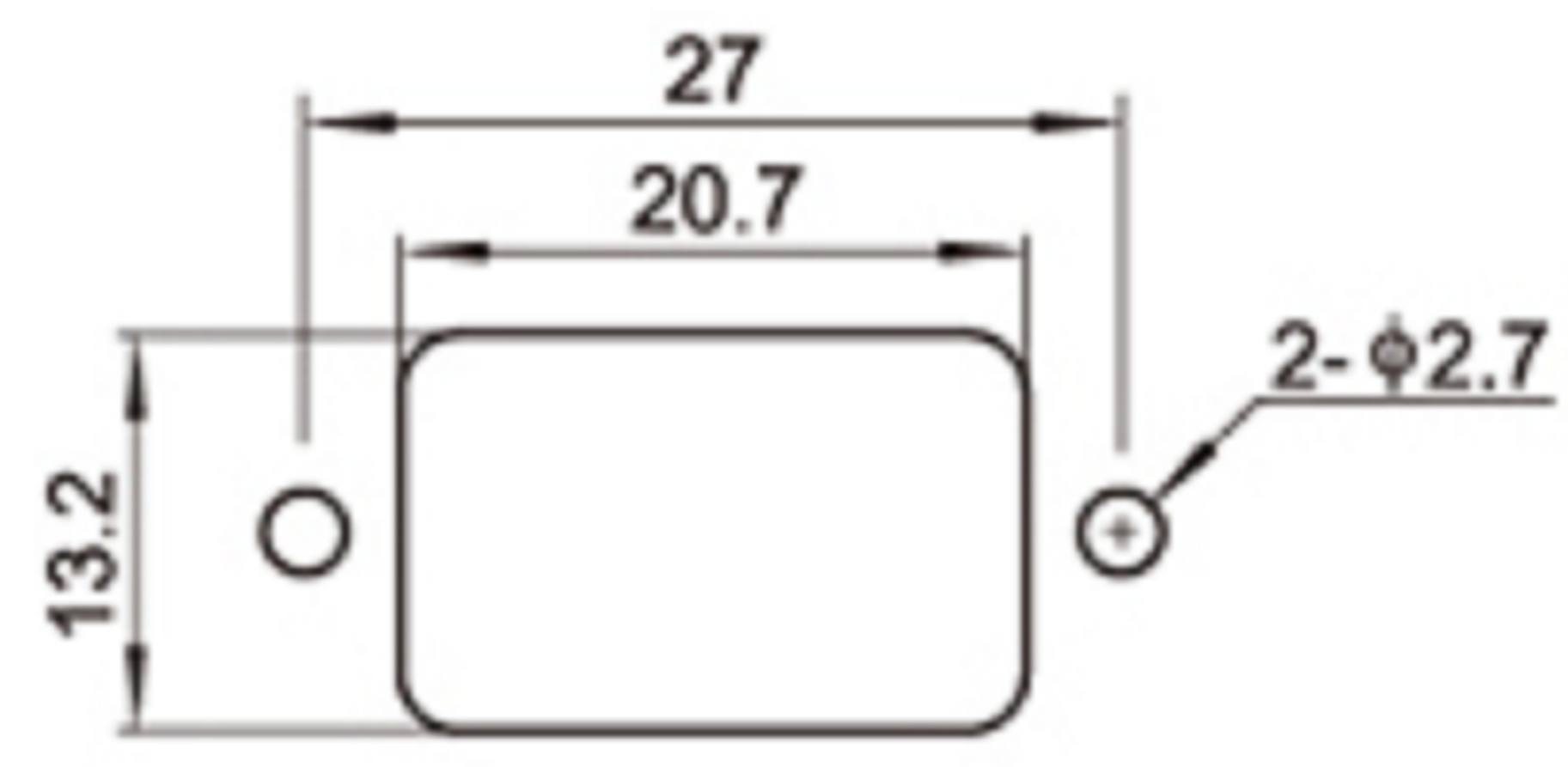
PANEL CUT-OUT
